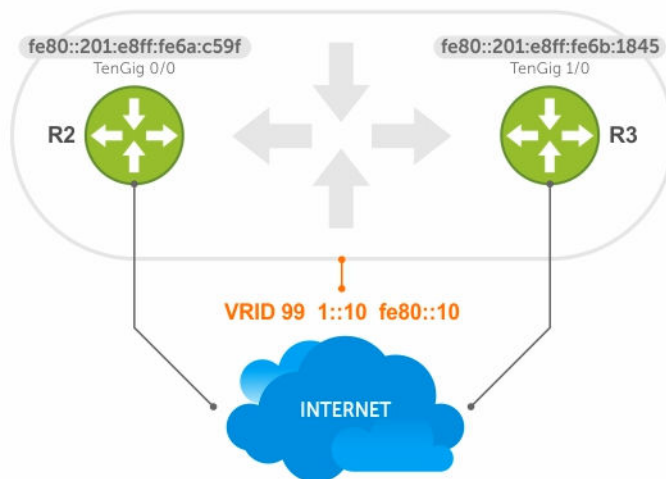
Figure 127. VRRP for an IPv6 Configuration
